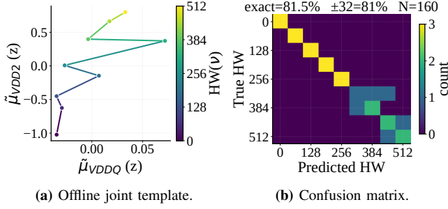
Figure 6: Hamming-weight recovery in the G = 0 mode: (a) the offline template, (b) the online per-line recovery.
