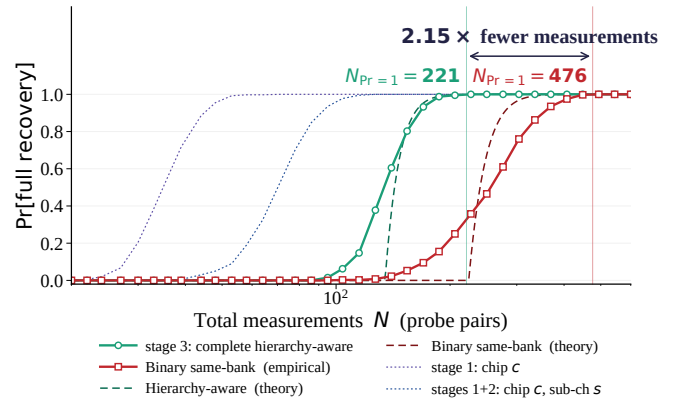
Figure 4: Recovery probability vs. measurements (Jetson TX2).
