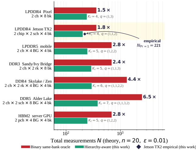
Figure 12: HOMARD-RE genericity across hierarchy depth.
