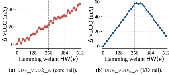
Figure 5: Hamming-weight response of the two DRAM rails. Both plots use amplification: the target line is replicated across contiguous cache lines and read repeatedly per trigger.
