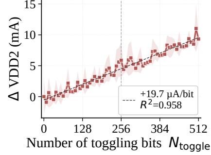
Figure 7: Linear HD response of DDR_VDD2_A to full-line bit toggling. The horizontal axis N_{\text{toggle}} is the number of toggling bits, i.e. the Hamming distance HD(G, V) of Equation 2
