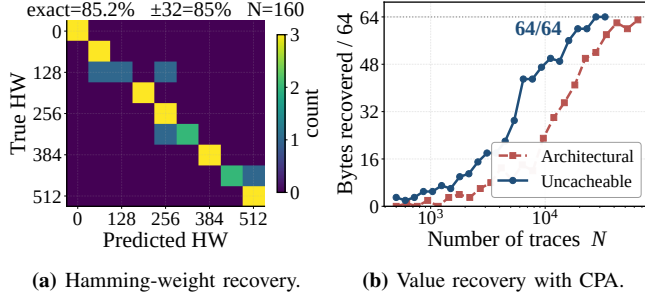
Figure 11: HOMARD-Data on uncacheable memory.
