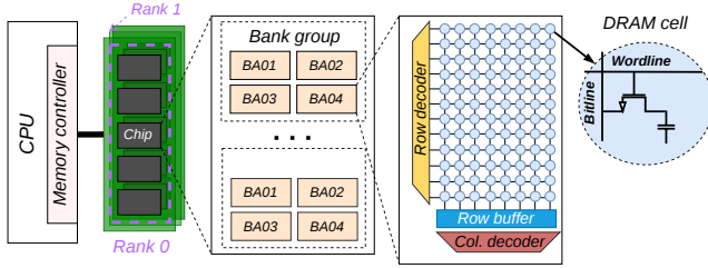
Figure 1: DRAM-based memory system organization.
