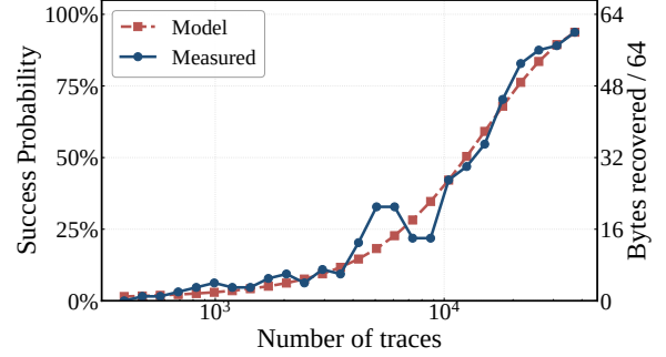
Figure 8: Blind byte recovery with CPA.
