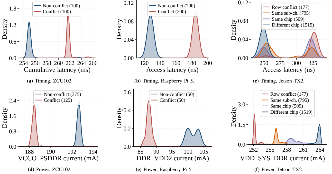
Figure 3: Timing (top) vs. power (bottom) on the three evaluation platforms. The parenthesized number in each legend entry is the number of probed address pairs falling in that class.
