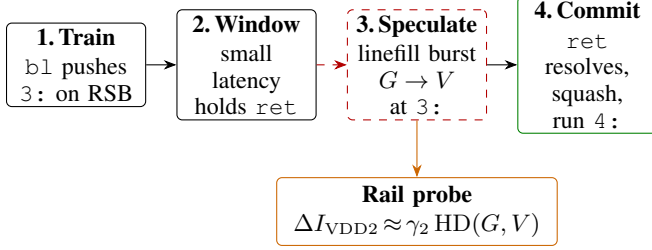
Figure 9: Spectre-RSB gadget for HOMARD-Data.
